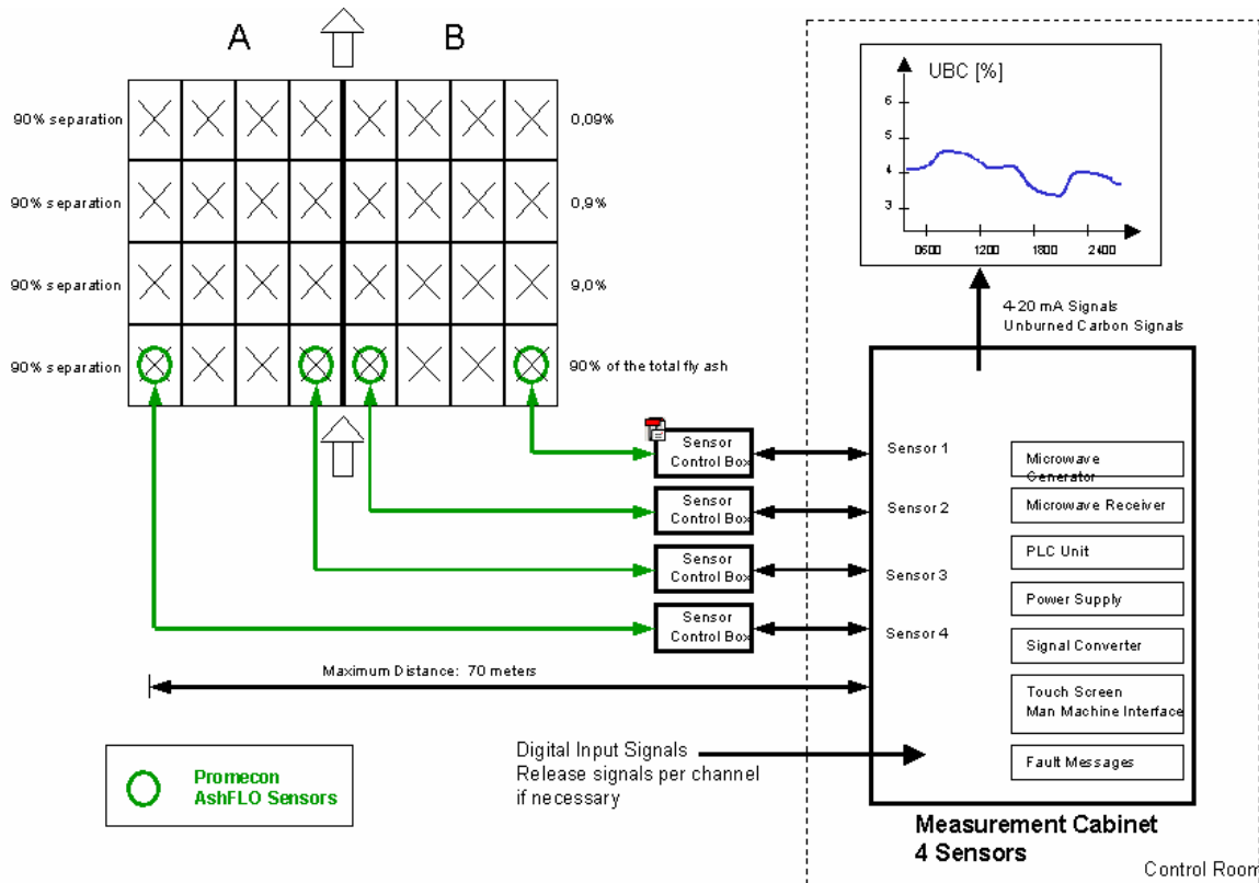
Figure 4: Typical utility boiler UBC system application
